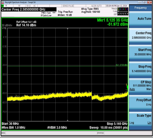
11N20SISO-Ant1-5280-30~5140-PASS
