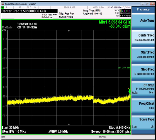
11A-Ant1-5260-30~5140-PASS
