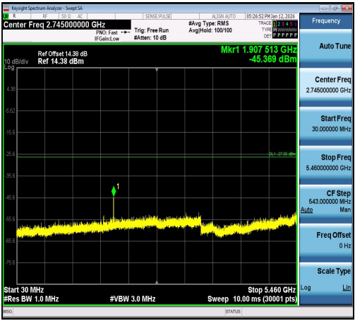
11N20SISO-Ant1-5700-30~5460-PASS
