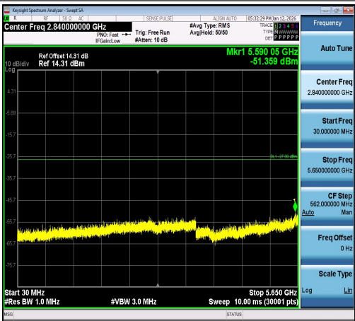
11N20SISO-Ant1-5745-30~5650-PASS
