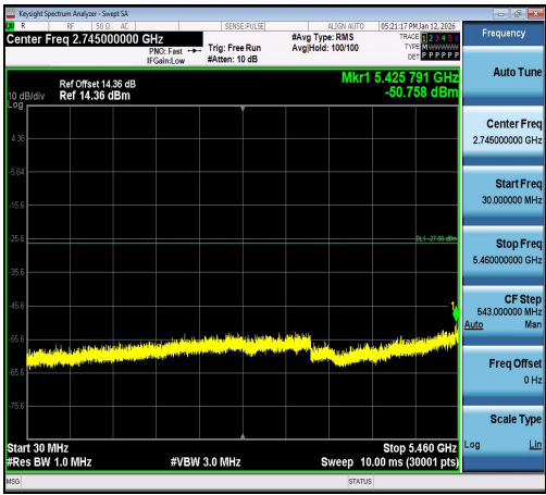
11N20SISO-Ant1-5580-30~5460-PASS
