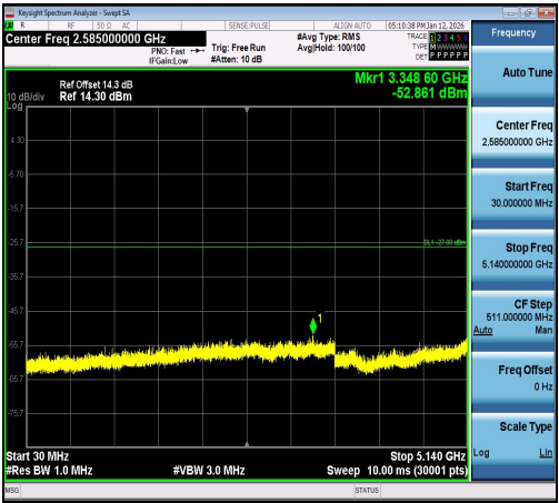
11N20SISO-Ant1-5320-30~5140-PASS
