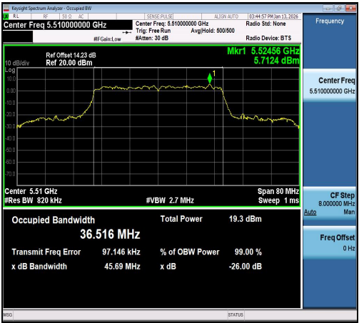
11AC40SISO-Ant1-5510
