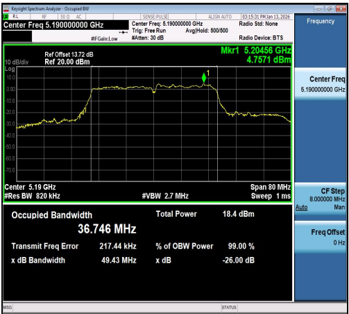
11AC40SISO-Ant1-5190
