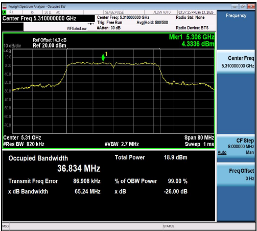
11AC40SISO-Ant1-5310
