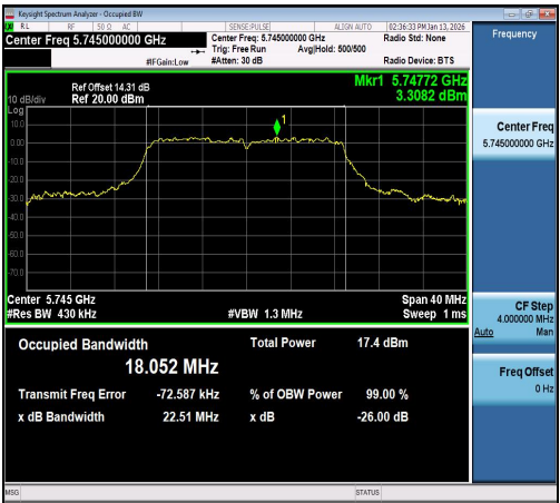
11AC20SISO-Ant1-5745
