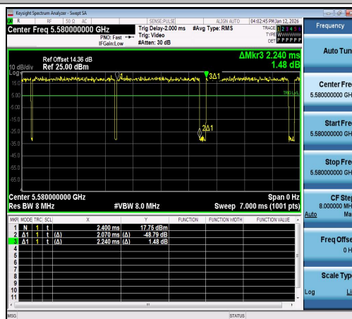
NTNV-11A-Ant1-5580
