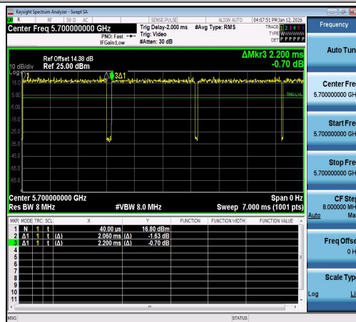
NTNV-11A-Ant1-5700
