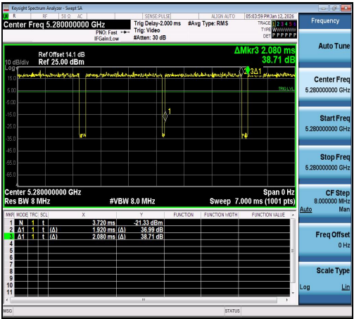
NTNV-11N20SISO-Ant1-5280
