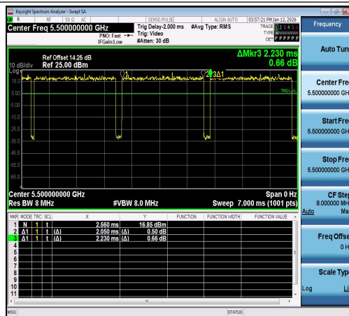
NTNV-11A-Ant1-5500
