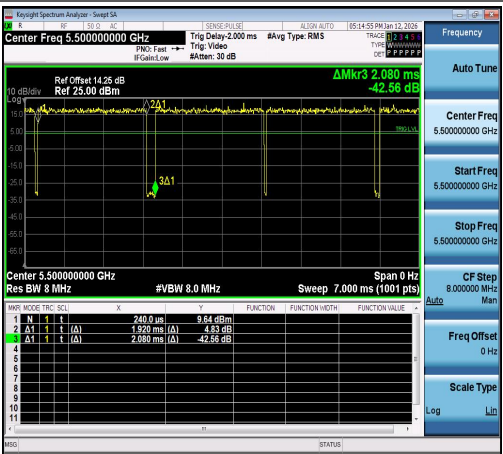
NTNV-11N20SISO-Ant1-5500
