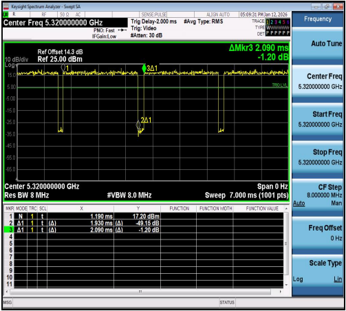
NTNV-11N20SISO-Ant1-5320
