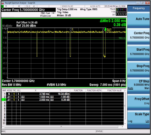
NTNV-11N20SISO-Ant1-5700
