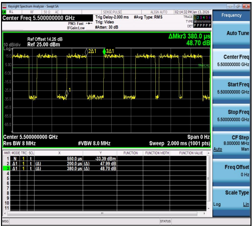
NTNV-11AC20SISO-Ant1-5500
