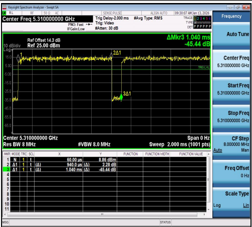
NTNV-11N40SISO-Ant1-5310
