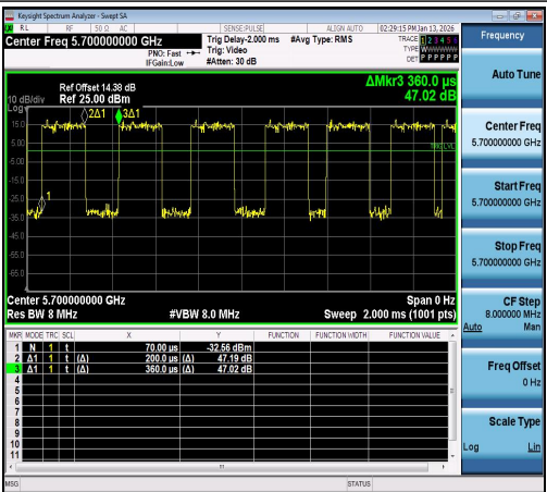
NTNV-11AC20SISO-Ant1-5700
