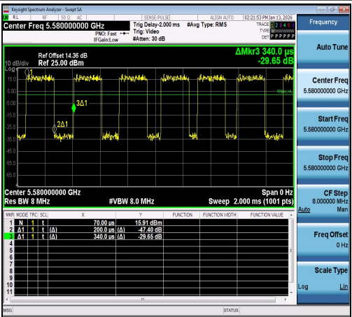
NTNV-11AC20SISO-Ant1-5580
