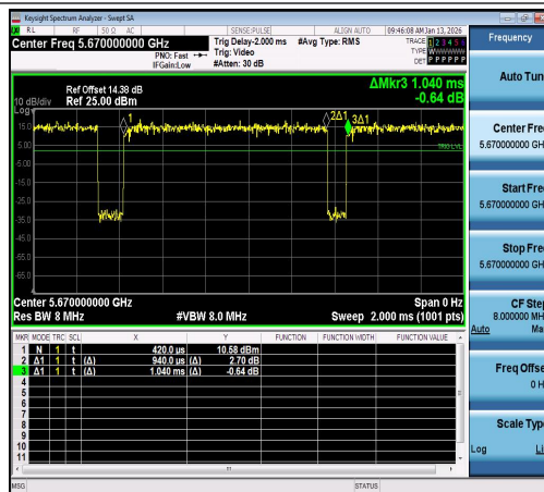
NTNV-11N40SISO-Ant1-5670
