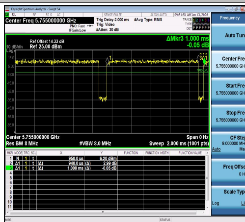
NTNV-11N40SISO-Ant1-5755
