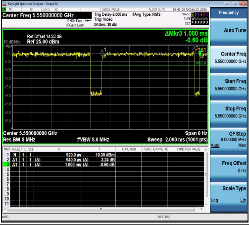
NTNV-11N40SISO-Ant1-5550
