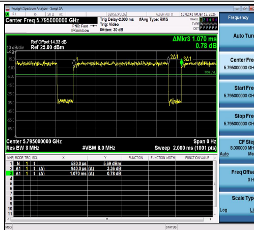
NTNV-11N40SISO-Ant1-5795
