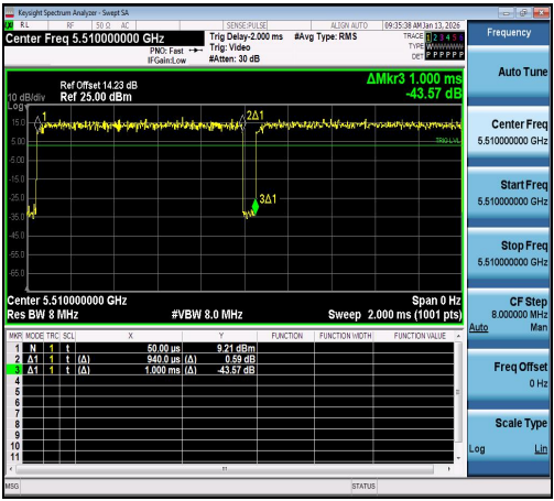
NTNV-11N40SISO-Ant1-5510
