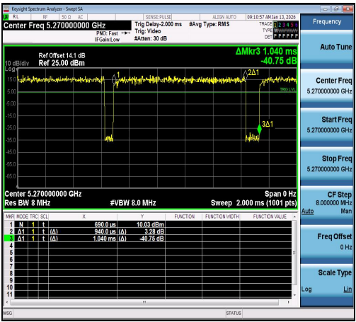
NTNV-11N40SISO-Ant1-5270
