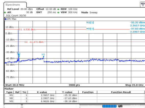
BLE_1M_Middle_Channel
