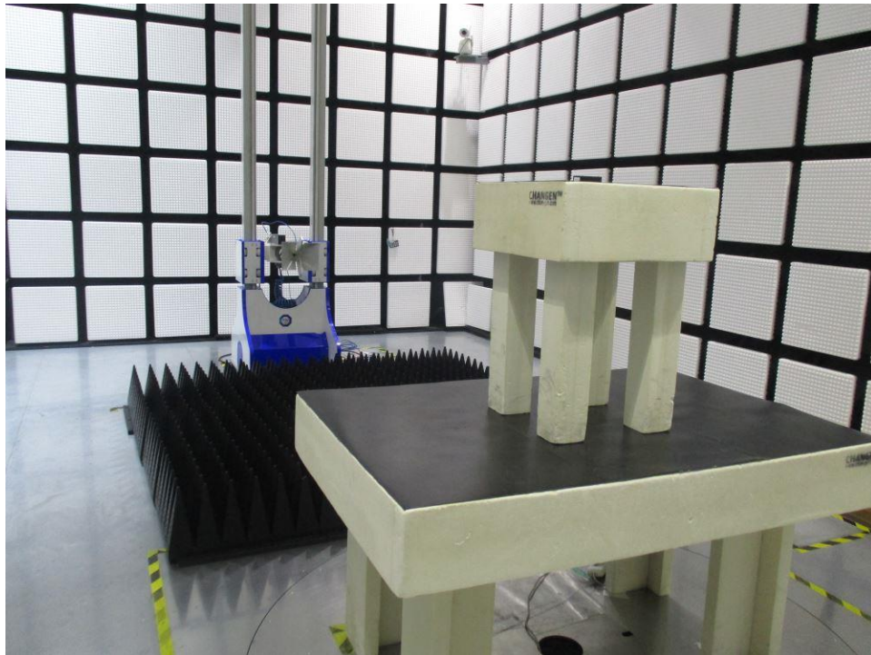
Spurious radiated emission Above 1GHz
