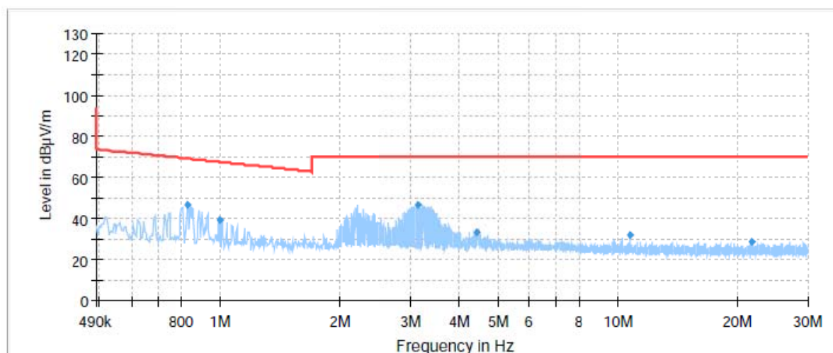
Radiates Emission from 490KHz to 30MHz
