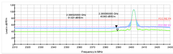
DH5-Channel 0: Peak + Average
