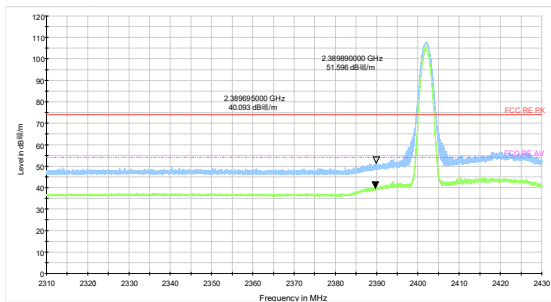
3DH5-Channel 0: Peak + Average
