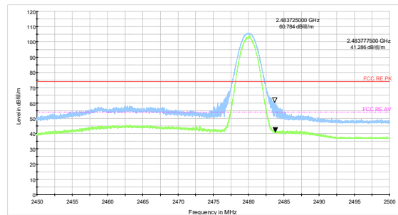
3DH5-Channel 78: Peak + Average
