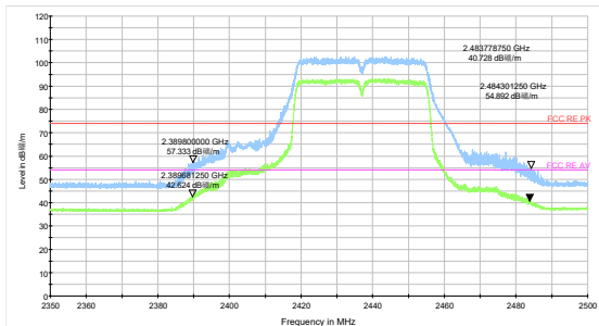
802.11n HT40 -Channel 6 Peak+ Average
