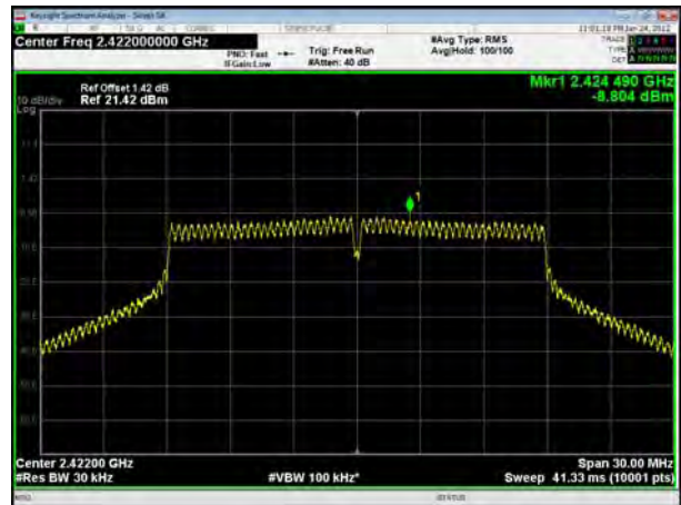
802.11n(HT20), Carrier frequency (MHz): 2422
