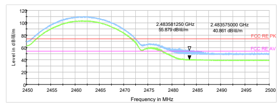
802.11b-Channel 11 Peak+ Average
