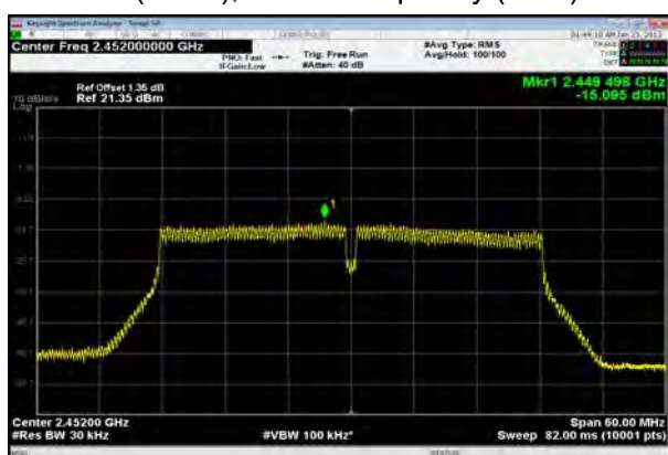
802.11n(HT40), Carrier frequency (MHz):2452
