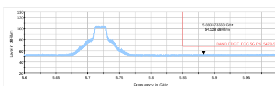
802.11n HT20-Channel 144: Peak
