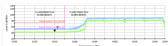
802.11ac VHT80 -Channel 42: Peak + Average
