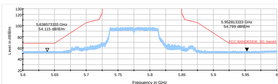
802.11ac VHT80- Channel 155: Peak
