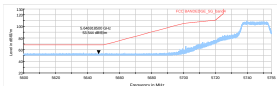
802.11a-Channel 149: Peak
