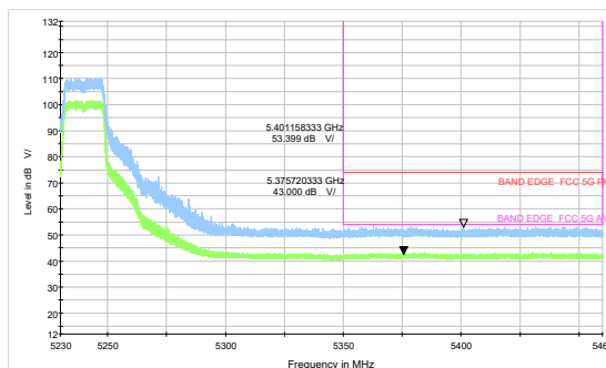
802.11a-Channel 48: Peak + Average
