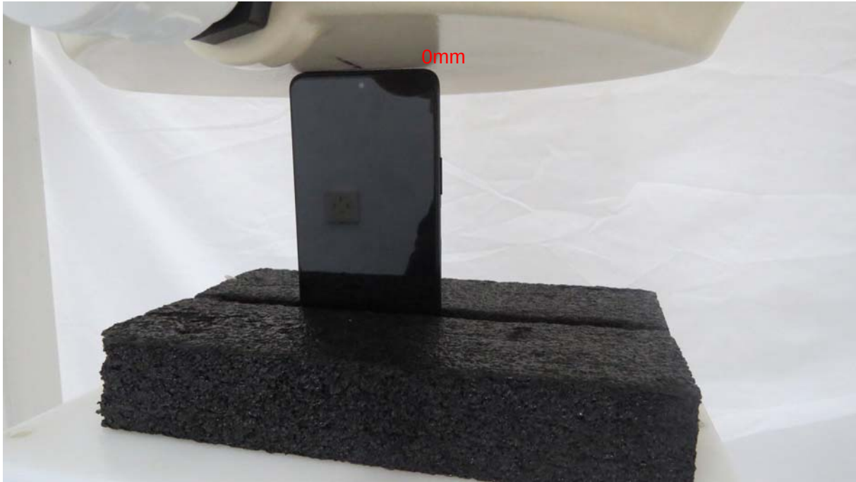
Picture 15: Top Edge, the distance from handset to the bottom of the Phantom is 0mm
