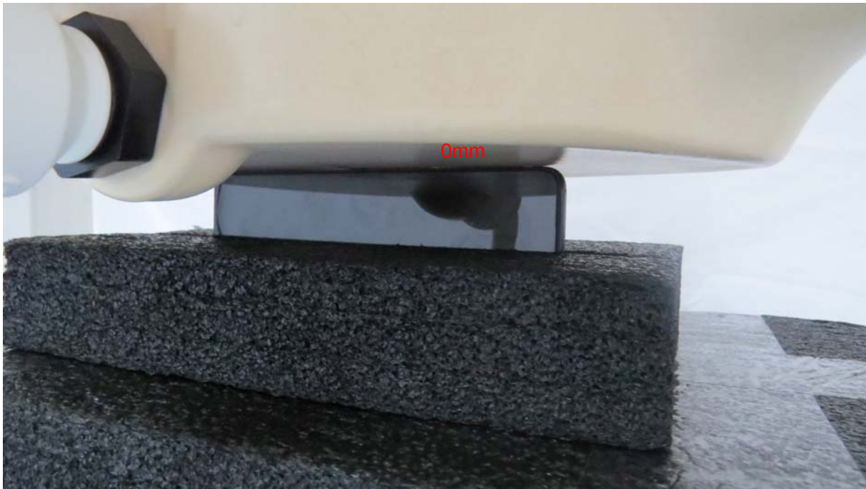
Picture 17: Left Edge, the distance from handset to the bottom of the Phantom is 0mm
