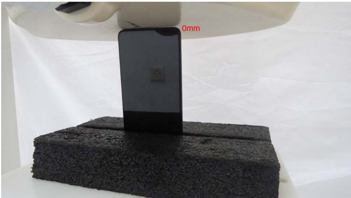
Picture 16: Bottom Edge, the distance from handset to the bottom of the Phantom is 0mm
