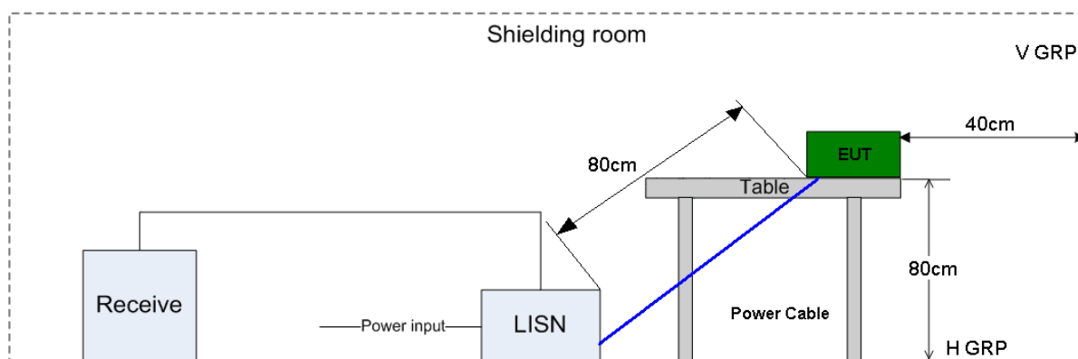
Figure 1. Test Set-up of conducted disturbance
