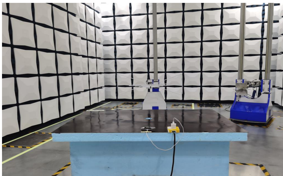
Radiated Spurious Emission (30MHz-1GHz)
