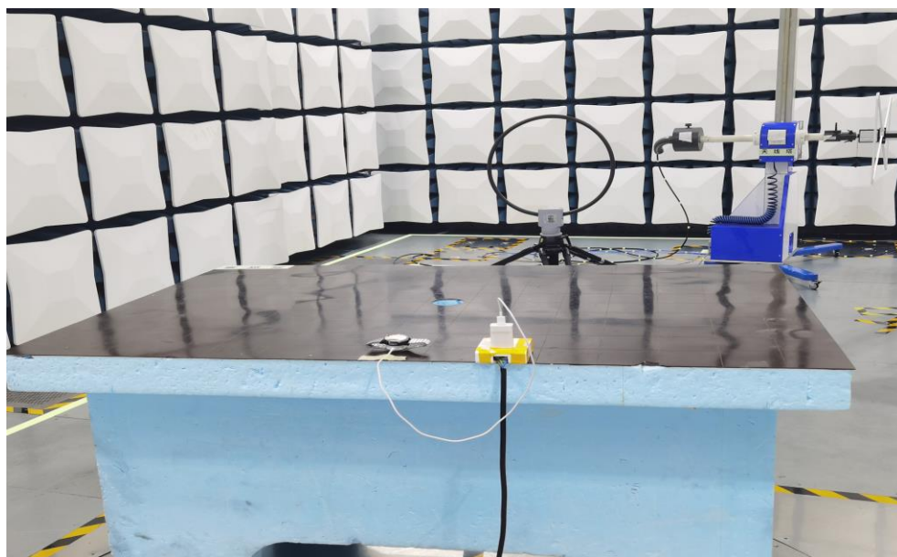
Radiated Spurious Emission (9K-30MHz)
