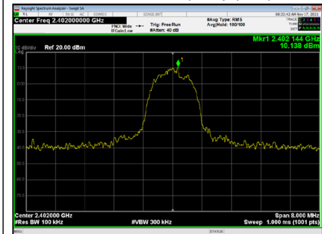
BT 3DH5 CH0, Carrier frequency (MHz): 2402
