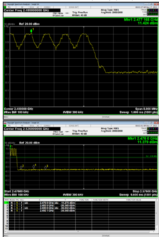
BT 2DH5 CH78, Carrier frequency (MHz): 2480
