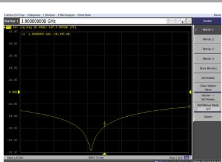
Return Loss Test-Head
