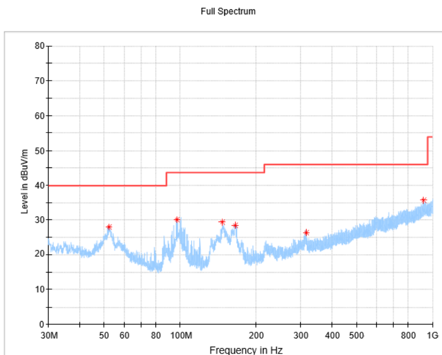
MEASUREMENT RESULT: QP Detector
