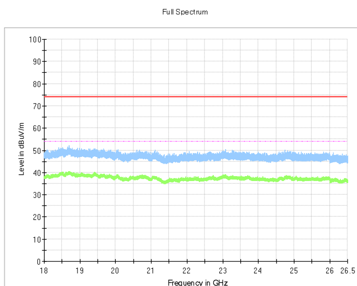
Worst case CH_2402- BLE_1M
