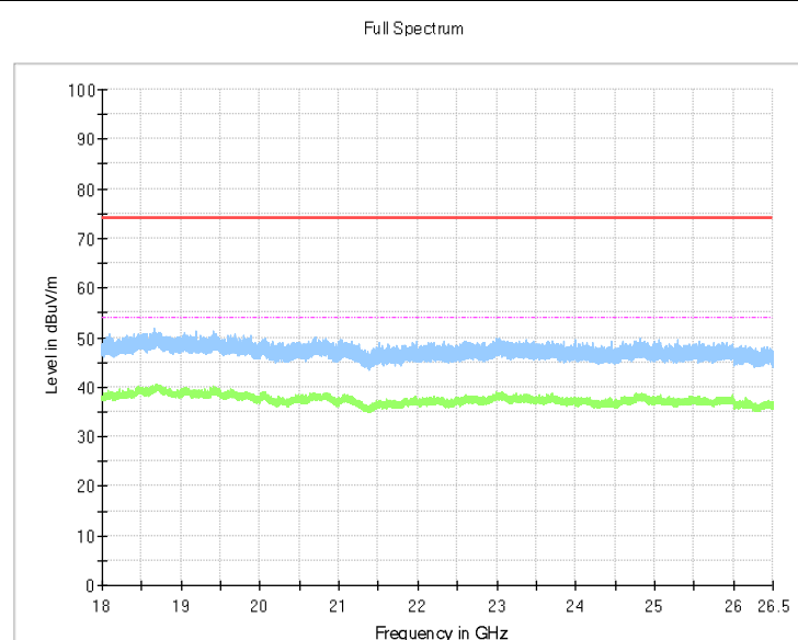
Worst case CH_2402- BLE_2M
