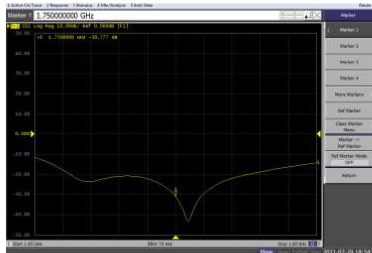
Return Loss Test-Head
