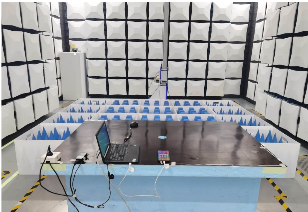
Radiated Disturbance Emissions (18GHz to 40GHz)
