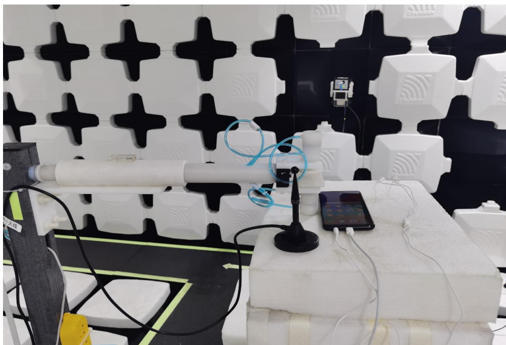
Radiated Spurious Emission (above 18GHz)
