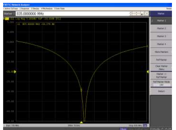
Return Loss Test-Body
