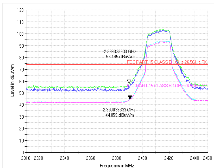
CH_2412(Band Edge)
