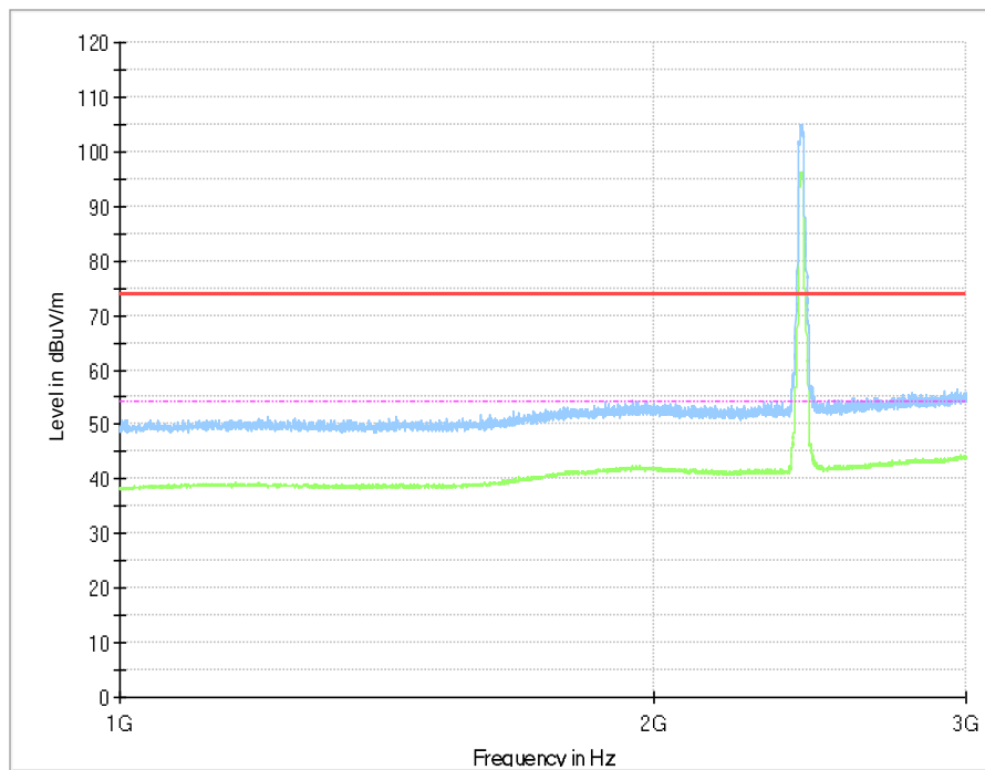
CH_2412(Band Edge)
