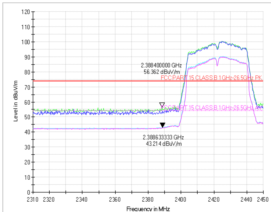
CH_2422(Band Edge)
