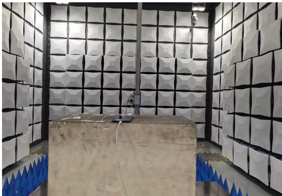
Radiated Spurious Emission (above 18GHz)
