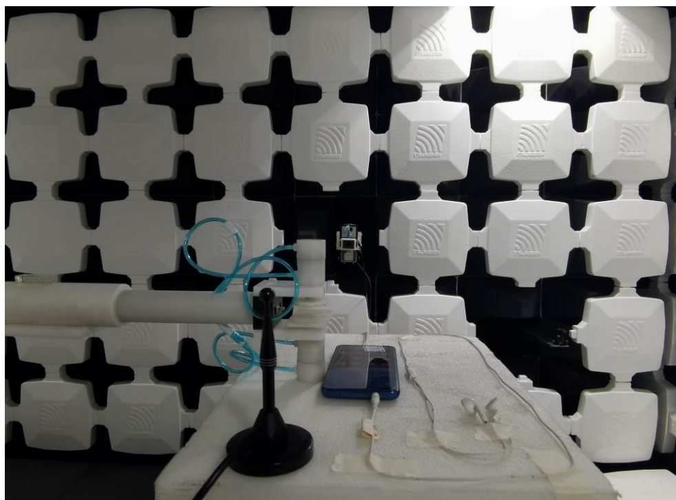
Radiated Spurious Emission (above 18GHz)
