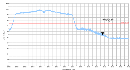
802.11n HT40 -Channel 8 Peak
