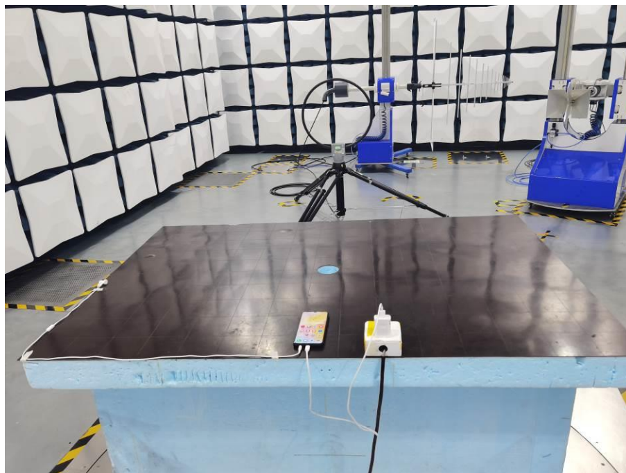
Radiated Spurious Emission (9K-30MHz)
