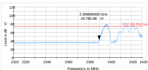
802.11g-Channel 2 Peak
