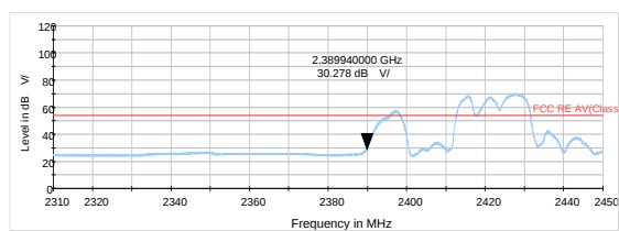
802.11n HT20 -Channel 3 Average
