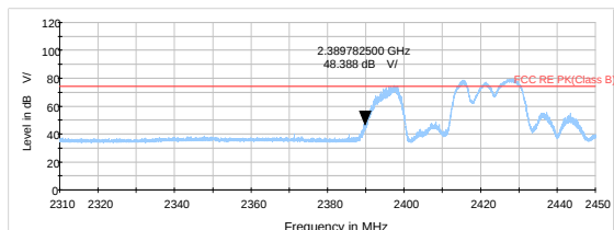
802.11n HT20 -Channel 3 Peak
