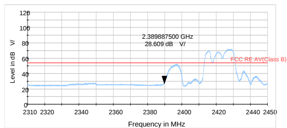
802.11g-Channel 3 Average
