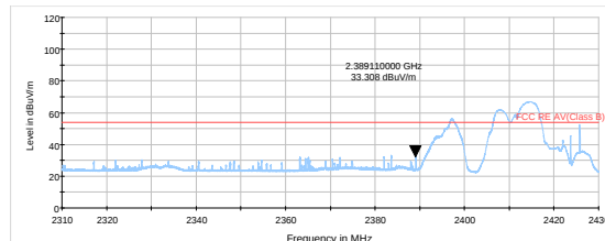
802.11b-Channel 1 Average
