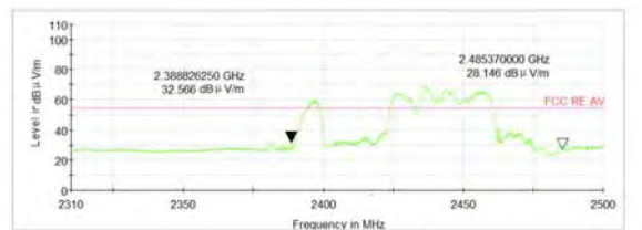
802.11n HT40 -Channel 7 Peak
