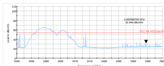
802.11b-Channel 11 Average
