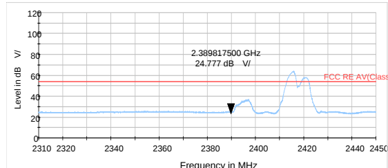
802.11n HT20 -Channel 2 Average
