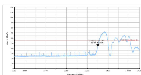
802.11g-Channel 1 Average
