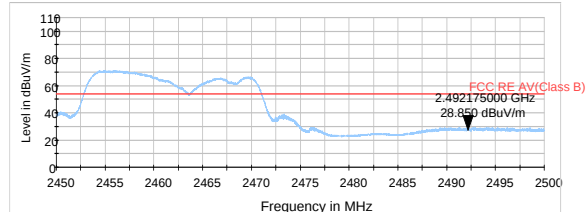
802.11g-Channel 11 Average
