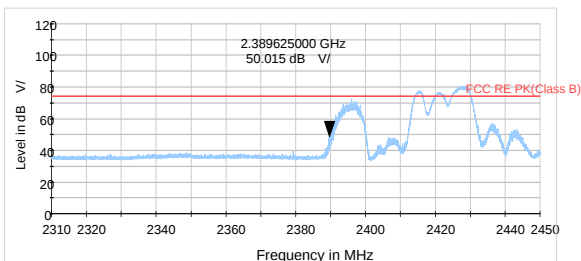
802.11g-Channel 3 Peak
