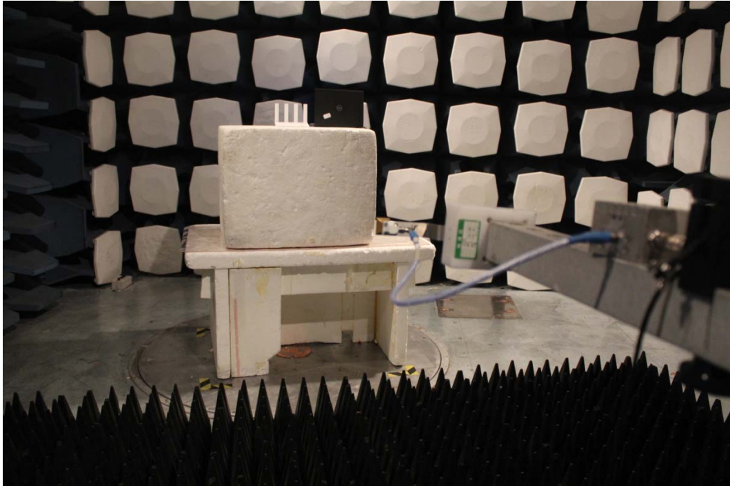
Picture 1 Radiated Emission Test Setup
