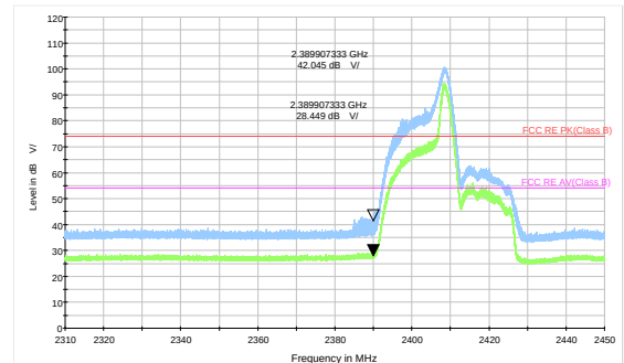
802.11n HT40 -Channel 2 Peak + Average
