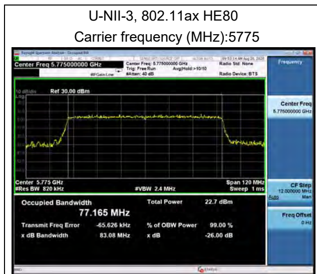
U-NII-3, 802.11ax HE80 Carrier frequency (MHz): 5775
