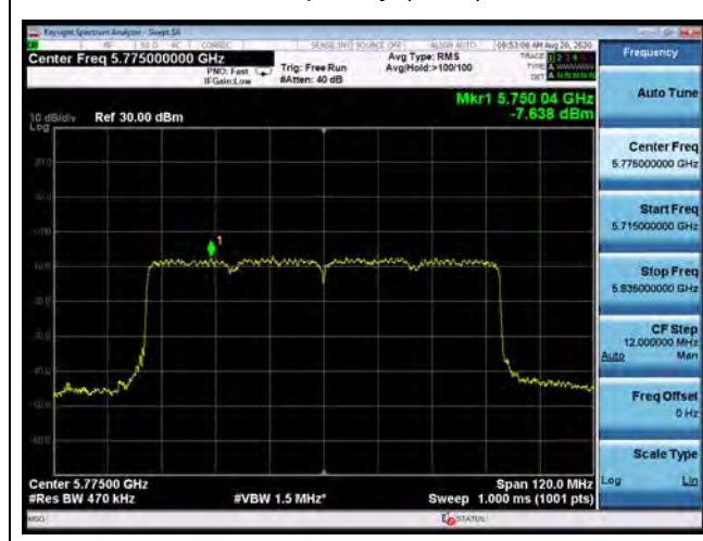
U-NII-3, 802.11ax HE80 Carrier frequency (MHz): 5775
