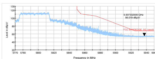
802.11ax HE40 Channel 159: Peak
