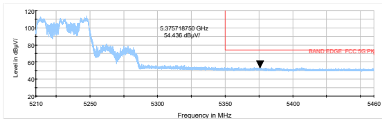
802.11ax HE40 Channel 46: Peak
