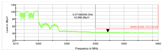
802.11ax HE40 Channel 46: Average
