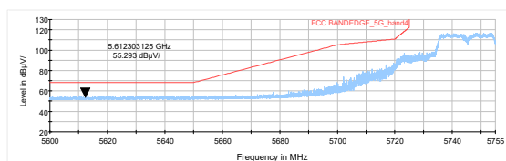
802.11ax HE40 Channel 151: Peak
