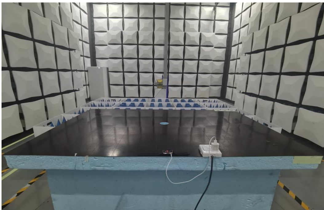
Radiated Emission (1GHz to18GHz)
