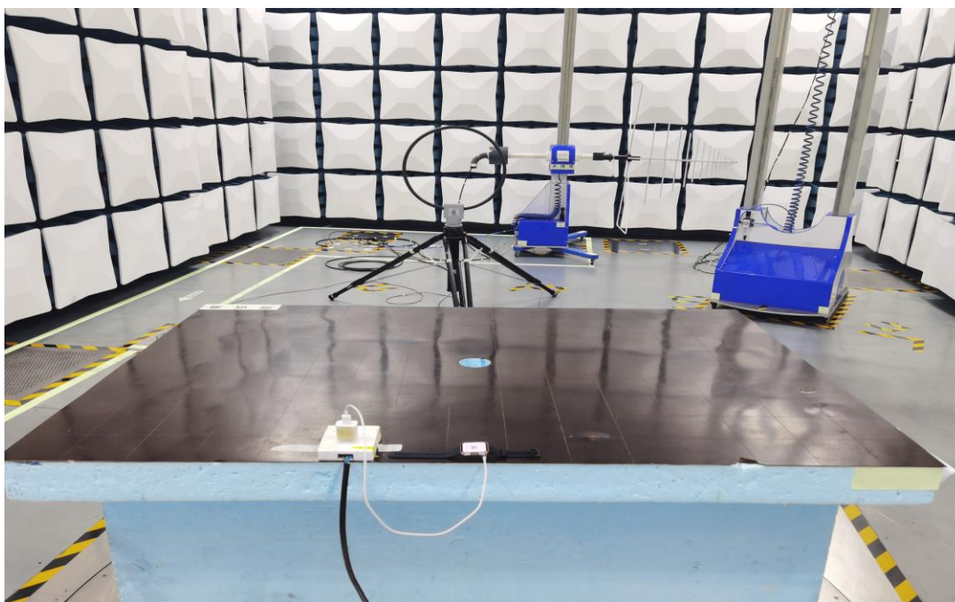
Radiated Spurious Emission (9K-30MHz)
