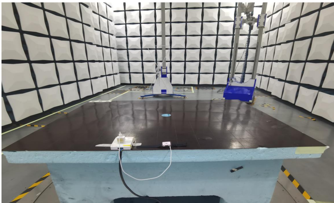
Radiated Spurious Emission (30MHz-1GHz)
