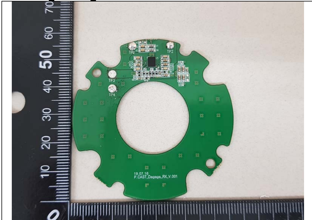
RX Board Tumbler Front
