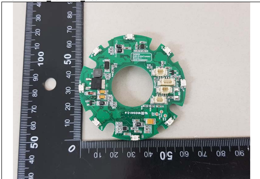
Main Board Tumbler Rear
