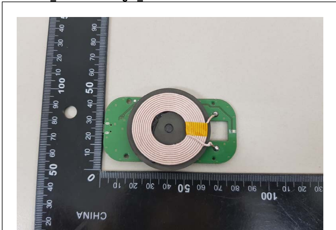
TX Board_Wireless Charger_Rear
