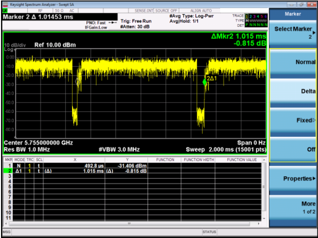
Ton+off
