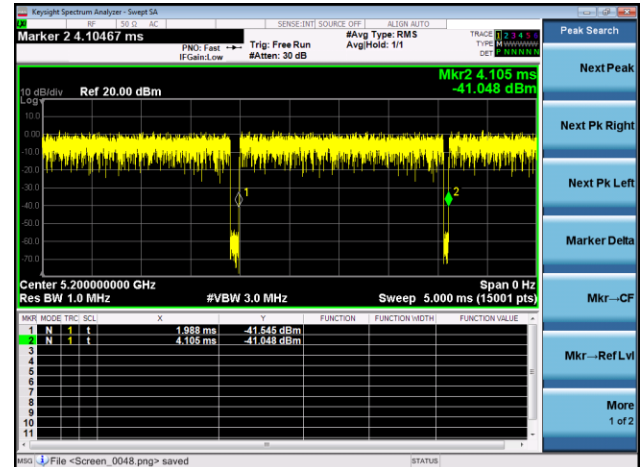
Ton+off
