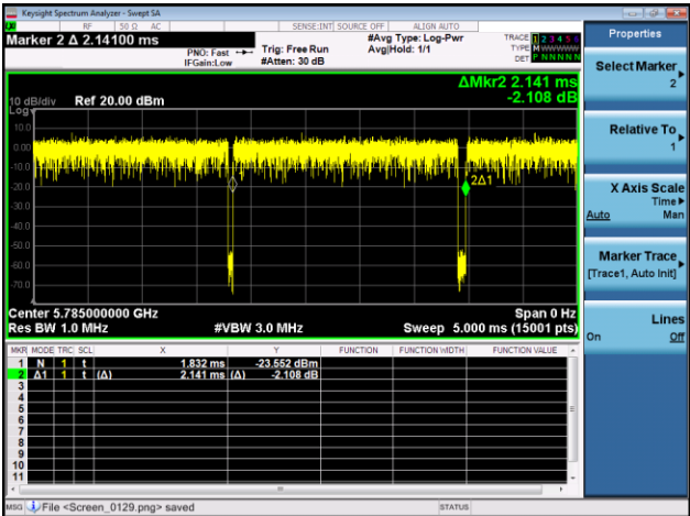
Ton+off
