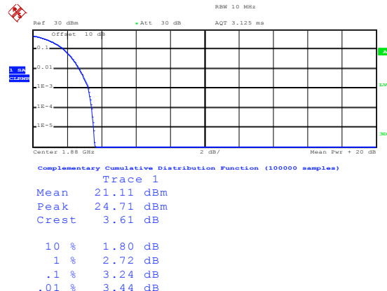
UMTS 1900 RMC
