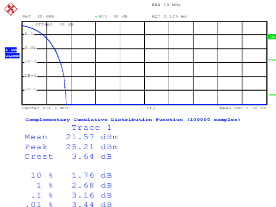
UMTS 850 RMC
