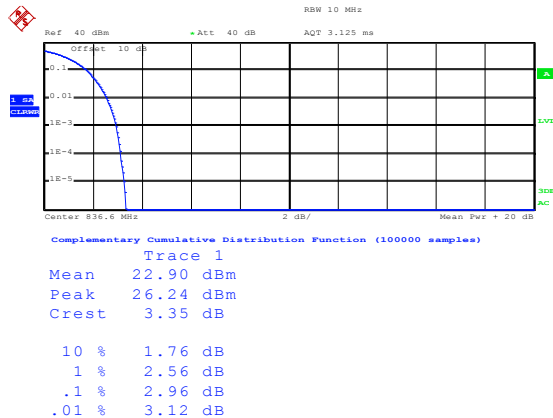
UMTS 850 RMC
