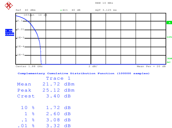
UMTS 1900 RMC
