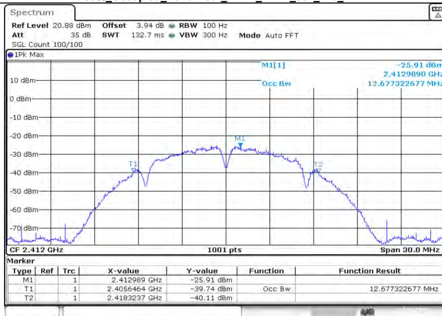
99%_Occupied_Bandwidth_NVNT_ANT1_802_11b_2412
