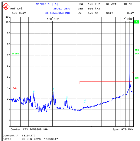
Antenna 1
