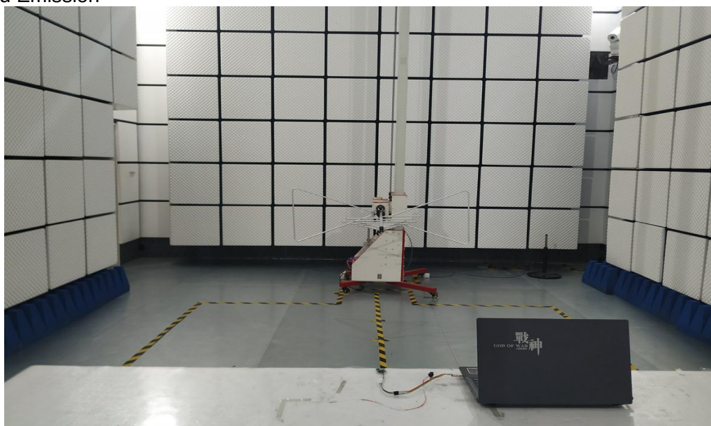
Radiated Emission
