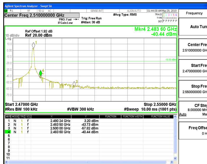
BLE_Ant1_High_2480
