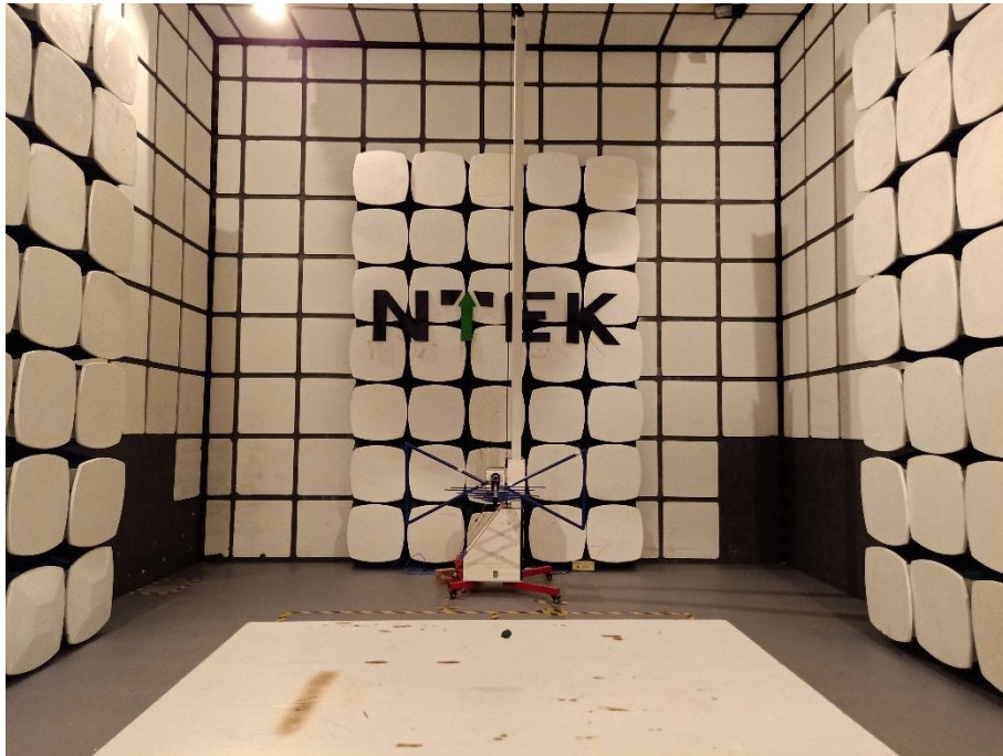
Radiated Measurement Photos (Left)
