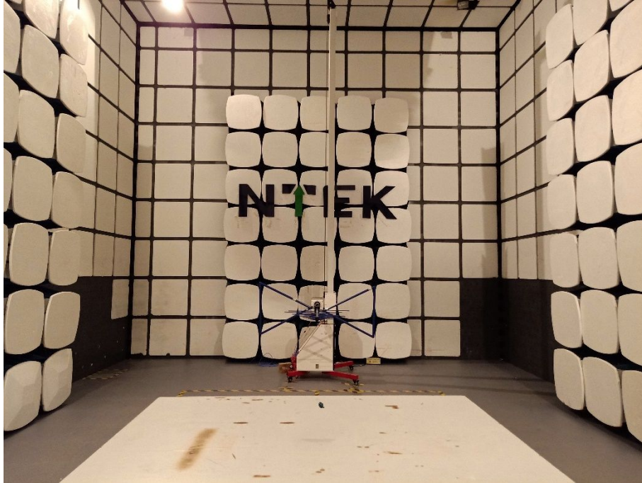
Radiated Measurement Photos (Right)
