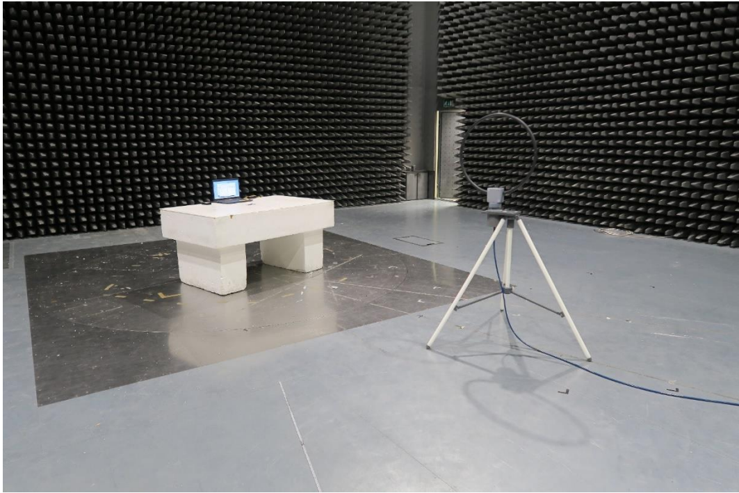
Photo 4.8.1 .....: Measurement of field strength of fundamental SA3-USB
