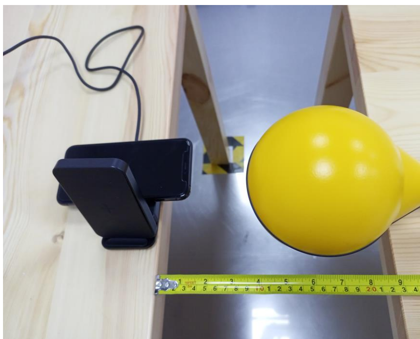
Test setup of D side (For Coil 2)
