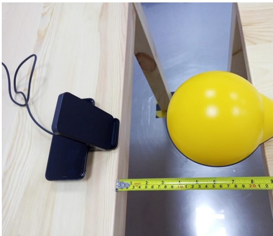
Test setup of A side (For Coil 2)
