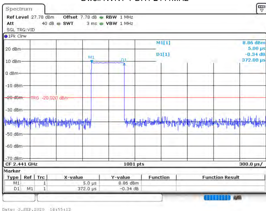
Dwell NVNT 1-DH1 2441MHz
