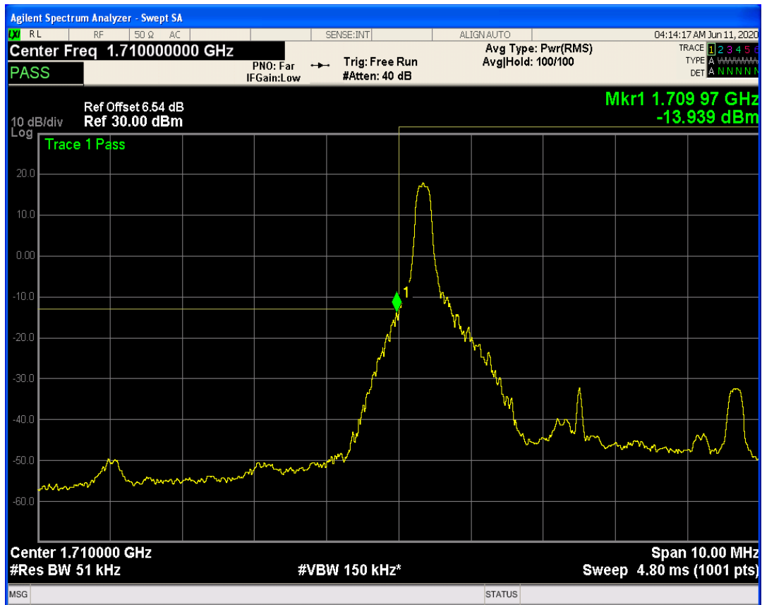
LTE Band66 QAM16 BW=5MHz Channel=131997 RB Size=1 Position=#Max
