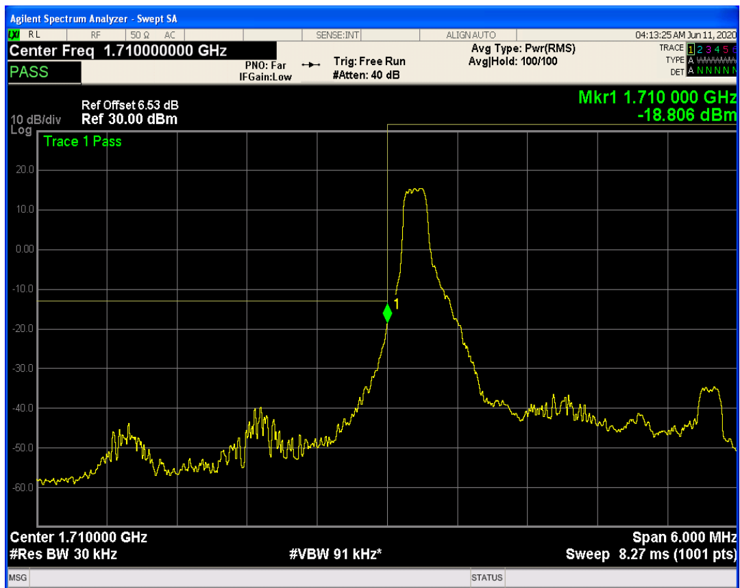
LTE Band66 QAM16 BW=3MHz Channel=131987 RB Size=1 Position=#Max
