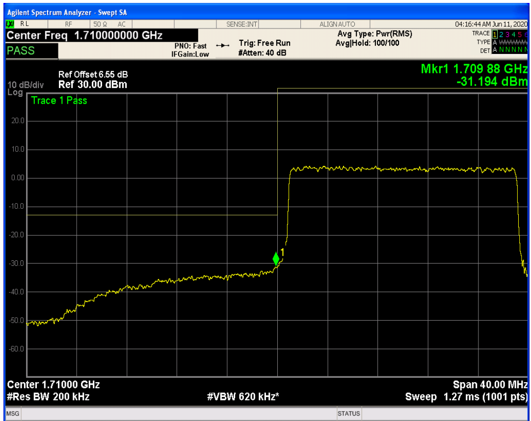
LTE Band66 QPSK BW=20MHz Channel=132072 RB Size=1 Position=#Max
