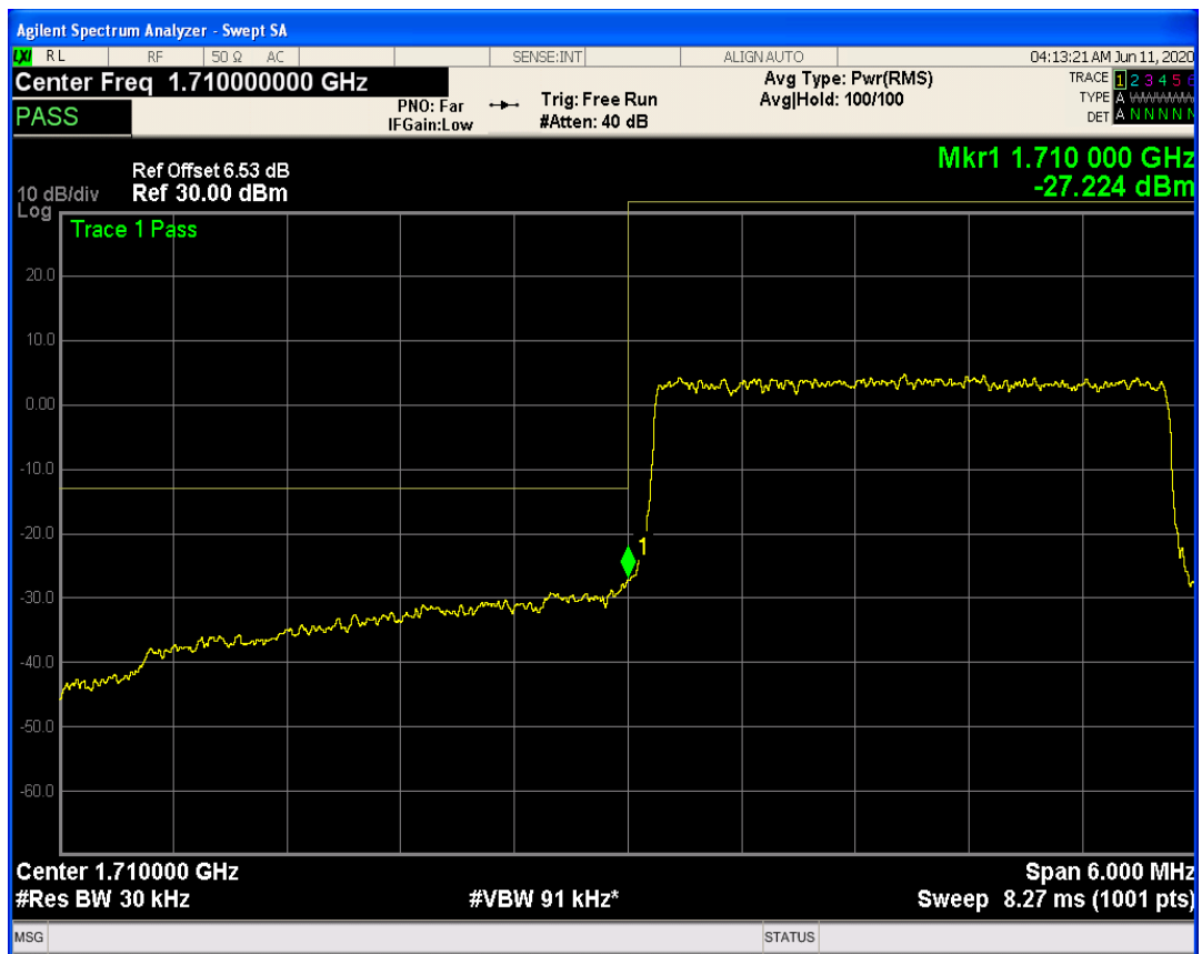
LTE Band66 QPSK BW=3MHz Channel=131987 RB Size=1 Position=#Max
