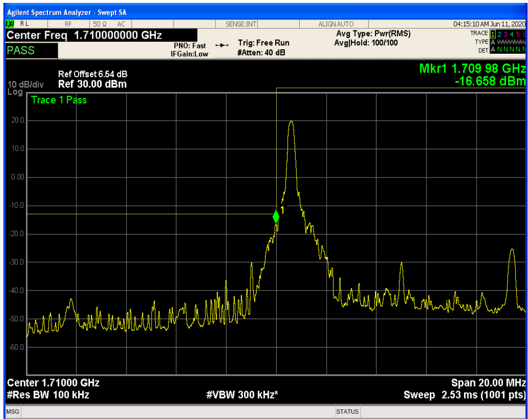
LTE Band66 QAM16 BW=10MHz Channel=132022 RB Size=1 Position=#Max
