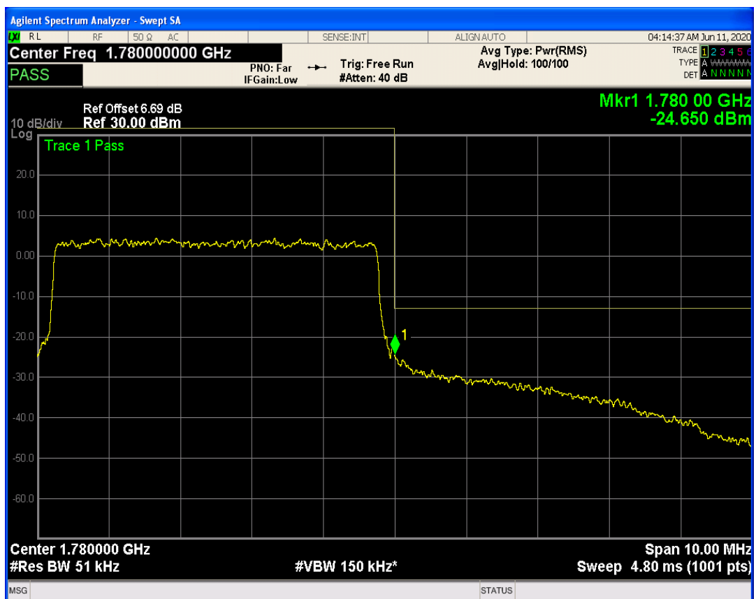
LTE Band66 QAM16 BW=5MHz Channel=132647 RB Size=1 Position=#Max
