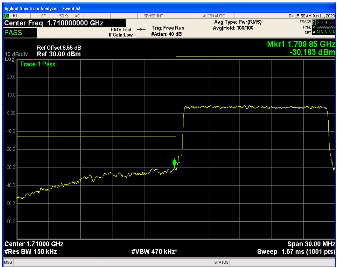
LTE Band66 QPSK BW=15MHz Channel=132047 RB Size=1 Position=#Max
