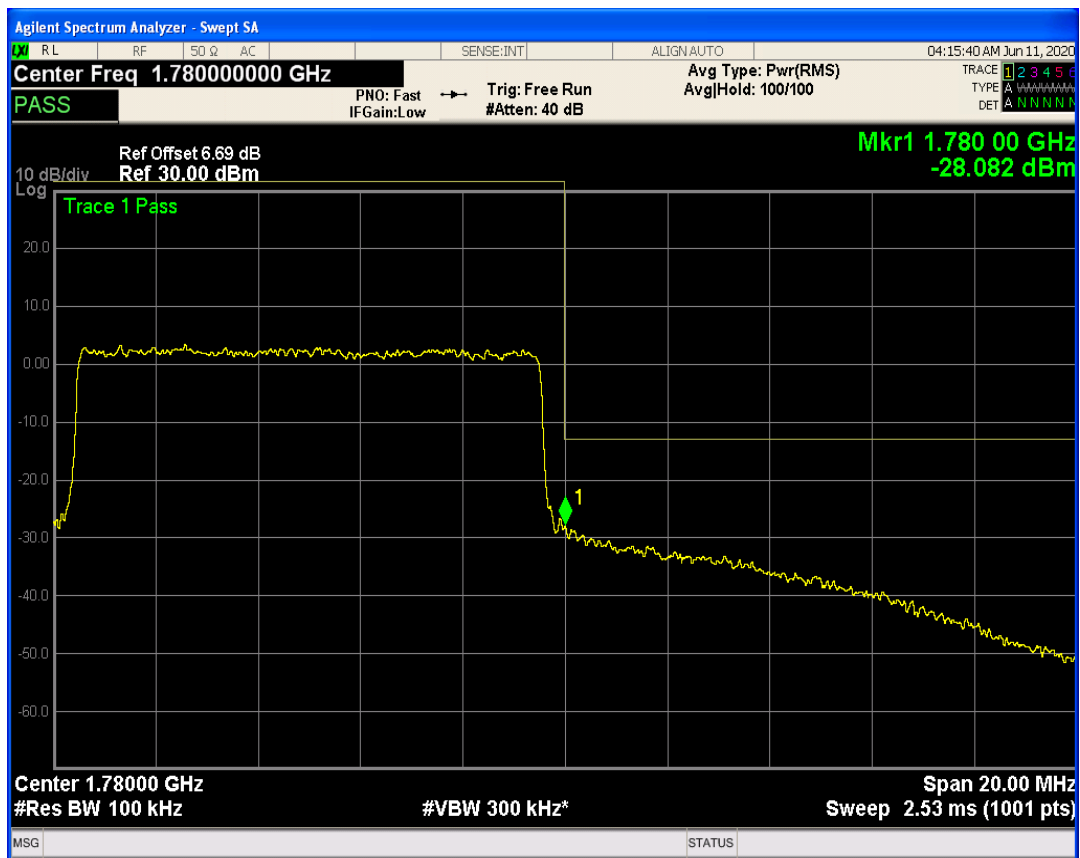
LTE Band66 QAM16 BW=10MHz Channel=132622 RB Size=1 Position=#Max
