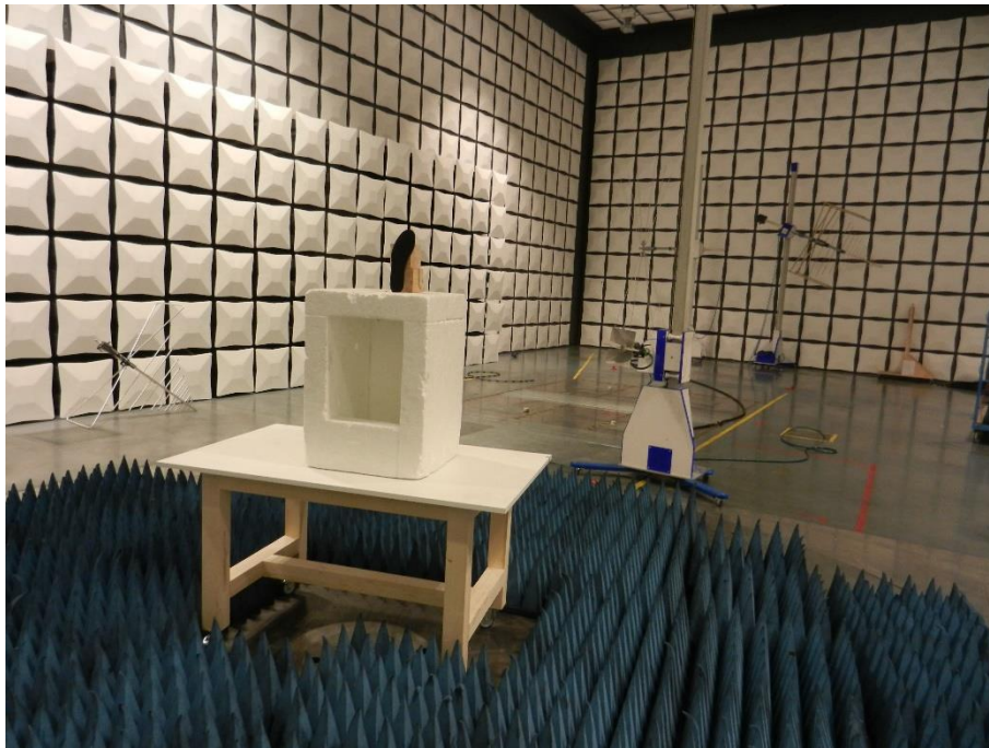
Radiated Emissions above 1 GHz, EUT upright
