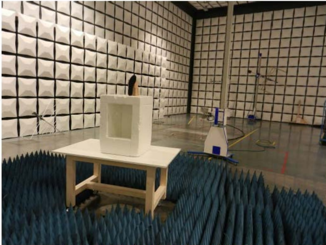
Radiated Emissions above 1 GHz, EUT upright
