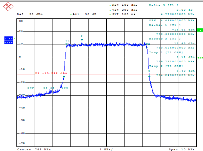
Band13-5MHz-QPSK-23230-25RB#0-4.496
