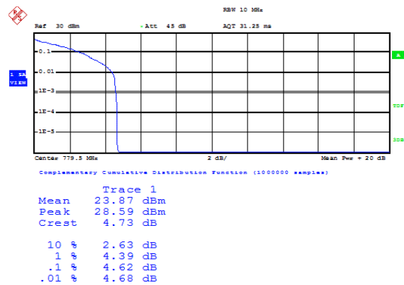
Band13-5MHz-QPSK-23205-1RB#0
