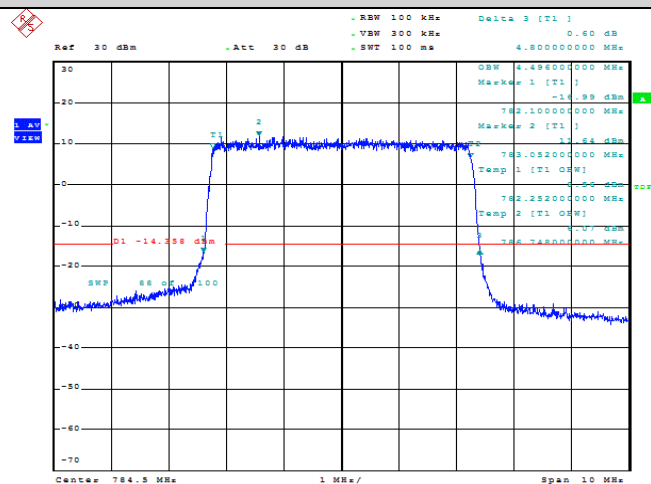
Band13-5MHz-QPSK-23255-25RB#0-4.496
