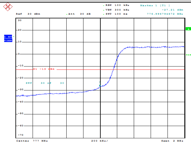
Band13-5MHz-QPSK-23205-25RB#0
