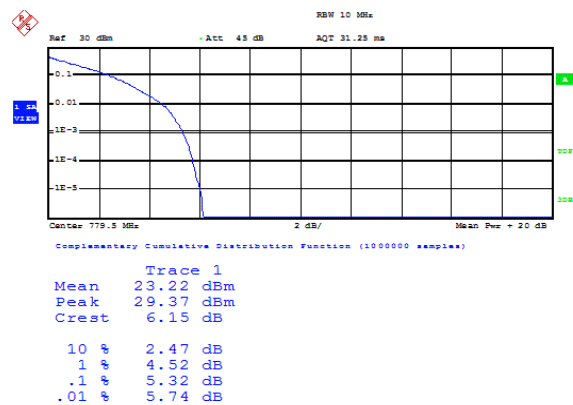
Band13-5MHz-QPSK-23205-25RB#0
