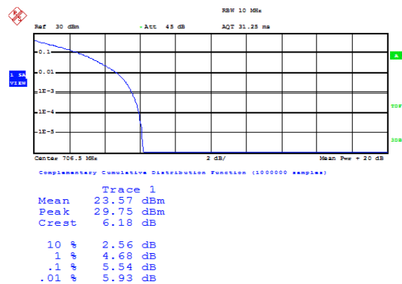
Band17-5MHz-QPSK-23755-25RB#0
