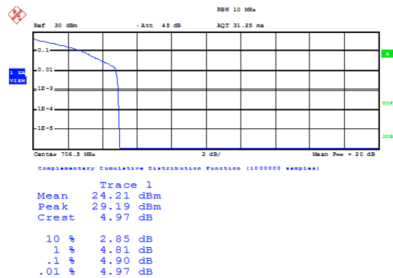
Band17-5MHz-QPSK-23755-1RB#0
