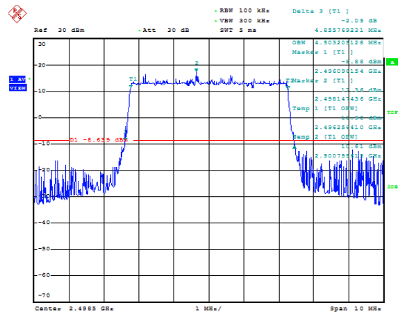
Band41-5MHz-QPSK-39675-25RB#0-4.503
