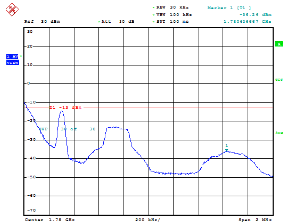
Band66-1.4MHz-QPSK-132665-1RB#0
