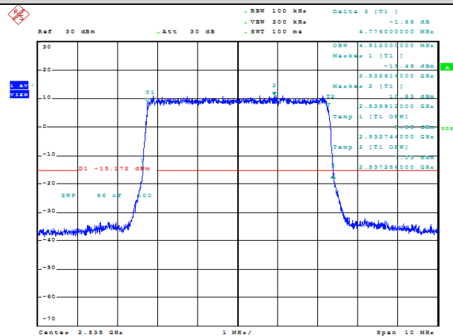
Band7-5MHz-QPSK-21100-25RB#0-4.512
